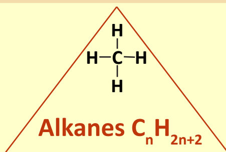
Methane
