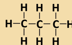
Propane
