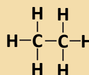
Ethane
